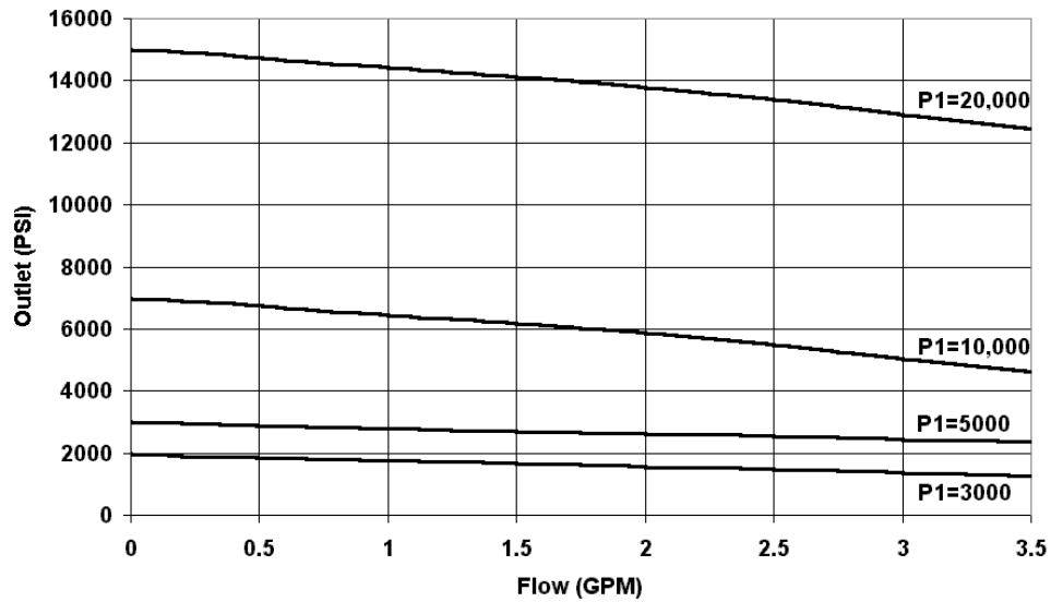
HR-1 Flow Characteristics
